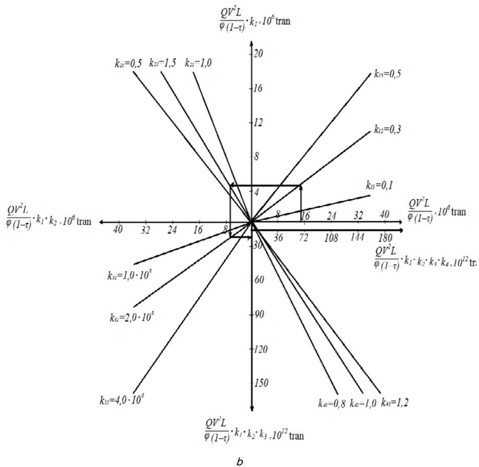
Fig. 2. Nomographs of determining a criterion of the generalized level of vehicle: a – defining the parameters of tran; b – refining the parameters of tran
